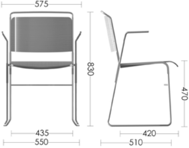
Lynn armchair Chromed metal frame 15x15 mm and Ø12 mm Seat and back made of beech veneer
